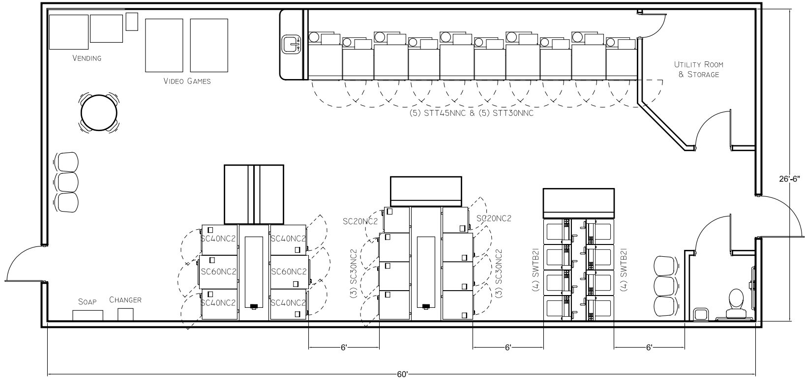
PRELIMINARY PLAN FOR CLEAN & BRIGHT LAUNDRY COMMERCIAL LAUNDRY SALES SCALE 1/8 IN = 1 FT 12MAY06 PROJECT NUMBER CLS-WI-0029
